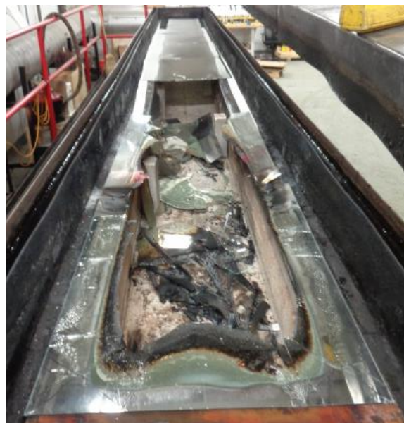
Photo No. 4 Exposed Surface of the Test Specimen (Post-test)
